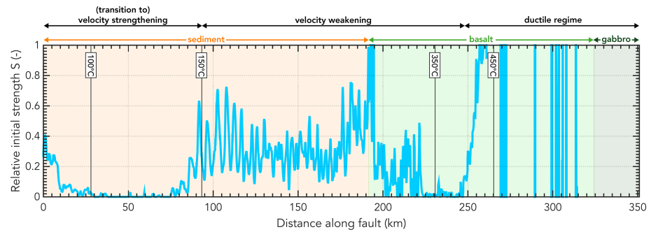
Figure D1. Relative strength S in the dynamic rupture model along the fault. Frictional regimes dependent on temperature are indicated with corresponding isotherms (solid black lines). Background colors represent the material through which the fault is going.
