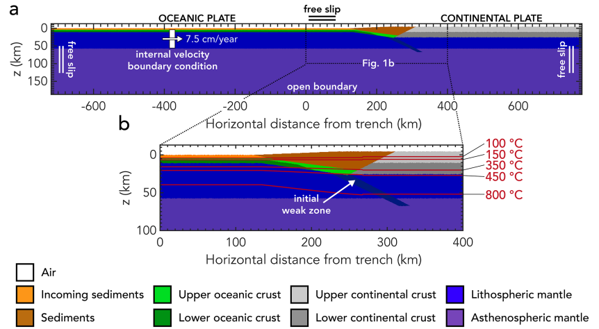
Figure 1. Complete (a) and zoomed (b) model setup of the geodynamic seismic cycle model with lithology (in color, see key), isotherms (red), and boundary conditions (white). Note that the future trench is located at (0,0) instead of (720,13) for easy comparison with the other figures in this work.
