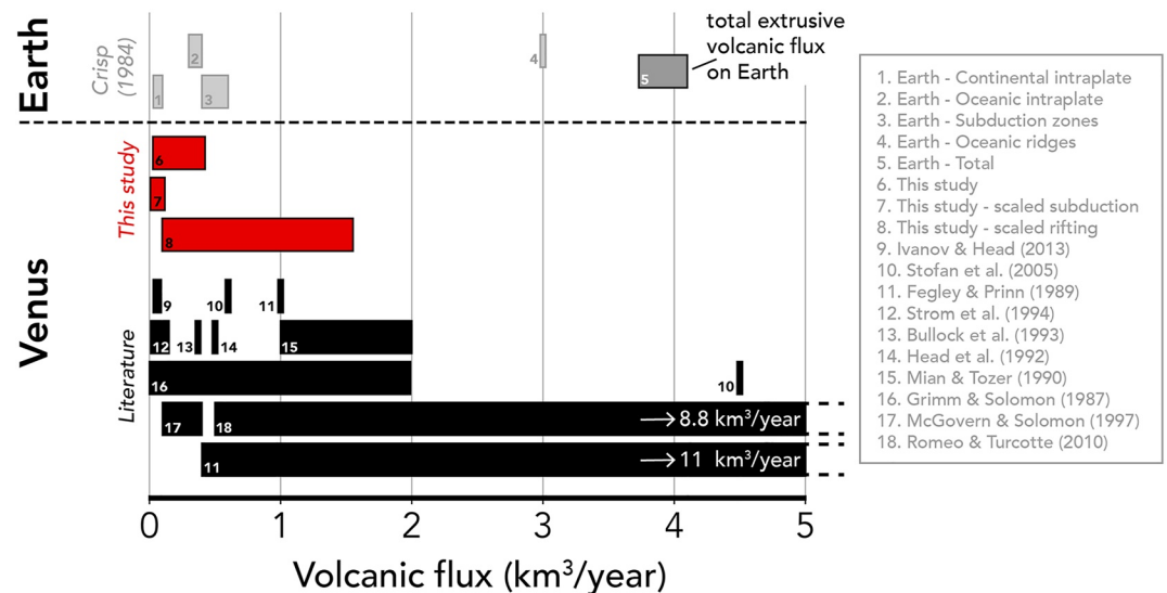
Figure 2. Comparison of the estimated annual extrusive volcanic flux on Venus based on the volcanic eruption frequency by Byrne and Krishnamoorthy (2022) using the corrected numbers calculated in this comment (6), including scaled subduction (7) and rifting volcanism (8), and previously published estimates of the extrusive volcanic flux of both Earth (1–5; Crisp, 1984) and Venus (9–18; Bullock et al., 1993; Fegley & Prinn, 1989; Grimm & Solomon, 1987; Head et al., 1992; Ivanov & Head, 2013; McGovern & Solomon, 1997; Mian & Tozer, 1990; Romeo & Turcotte, 2010; Stofan et al., 2005; Strom et al., 1994).
